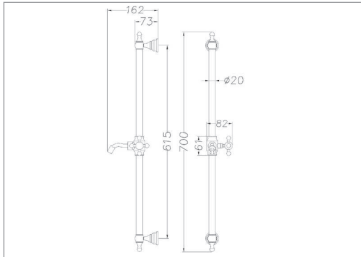
Lichfield Shower Rail kit, handset and hose
