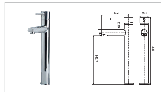
(For use with Regent Bay Composite top 1 tap hole) Chrome EX40000100
