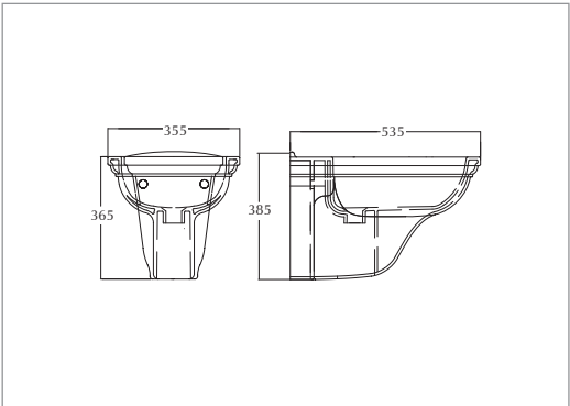
Wall-hung bidet (supplied without supporting brackets) (1 tap hole) White RD1BH11030
