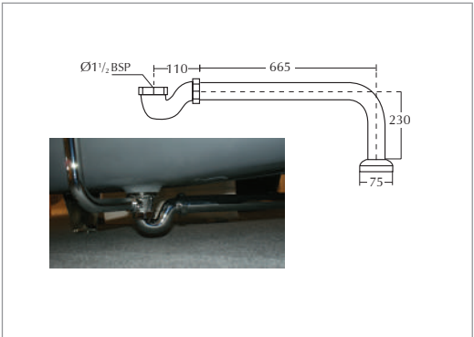
Roll top S trap low seal
