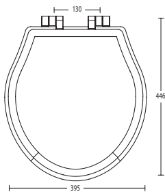
Regent solid wood toilet seat - with soft-close hinge Supplied with seat lid lift handle in the box
