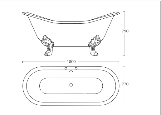
Sheraton double ended slipper bath (Supplied with Lion foot)
