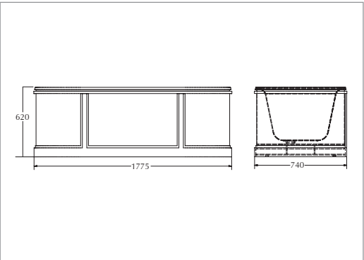
King Charles bath*
