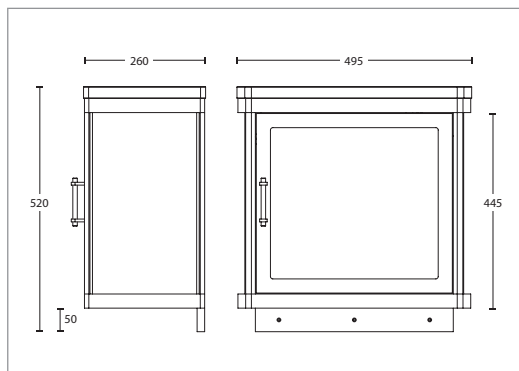
Carlyon cloak vanity basin
