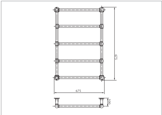
Lund 920x600 wall radiator** Water only
