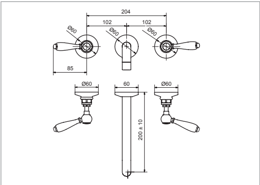
3 hole wall mixer
