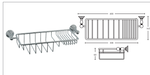
Richmond shower tidy wall mounted
