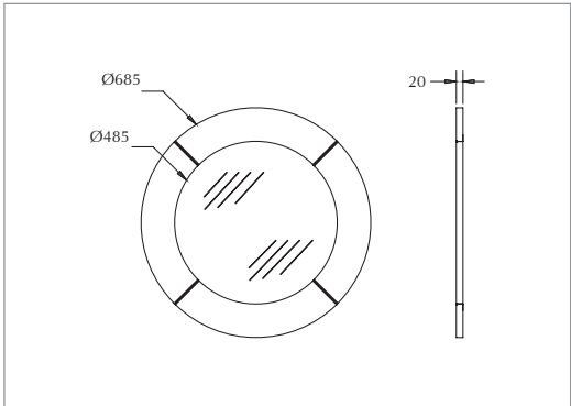
Carlyon Bay mirror - 685mm (with chrome strip detail) Sea Mist BAYMR00164
