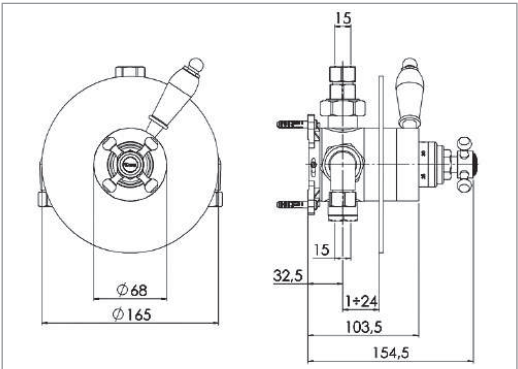
Concealed Westminister thermostatic control valve (White controls) SINGLE WATER OUTLET
