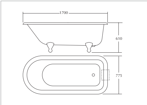
Waldorf single ended bath (Supplied with Ball & Claw feet)
