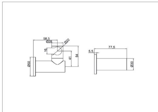
Lichfield shower Handset wall bracket
