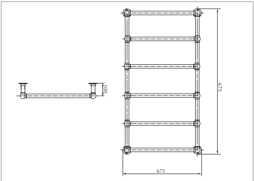
Lund 1450x500 wall radiator** Water only
