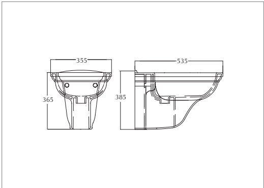
Wall-hung bidet (supplied without supporting brackets) (1 tap hole) White CR1BH11030
