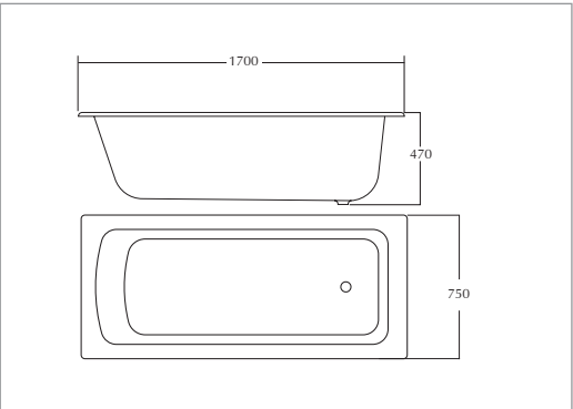
Harrington single ended cast iron bath (Supplied without bath panels)
