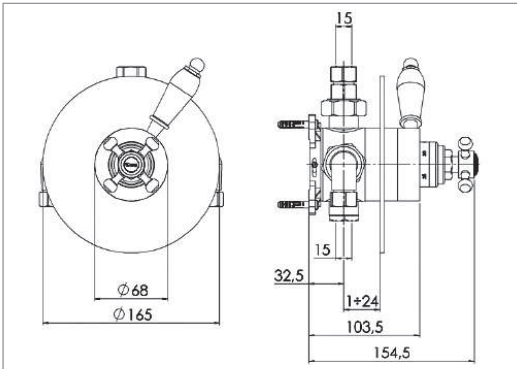
Concealed Westminister thermostatic control valve (Black controls) SINGLE WATER OUTLET
