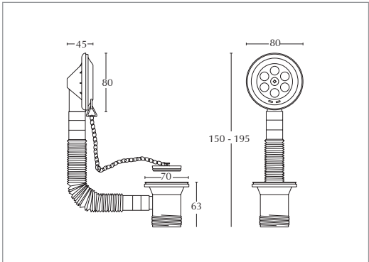
Tidy plug standard bath waste with plug and chain For use with acrylic baths and Harrington bath
