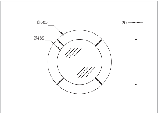
Carlyon Bay mirror - 685mm (with chrome strip detail) Matt Black BAYMR00160
