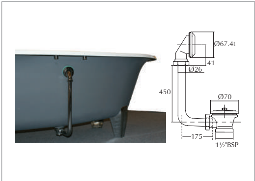
Exposed bath waste
