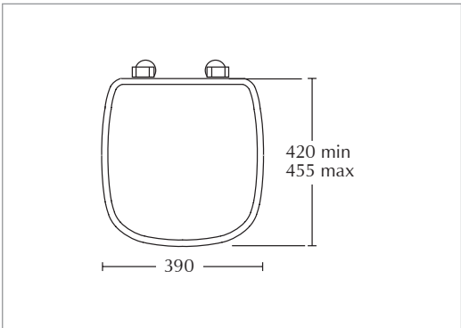
Radcliffe painted toilet seat - with soft-close hinge Supplied without seat lid lift handle
