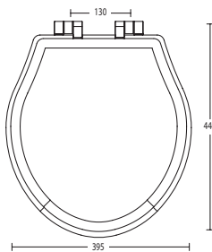
Regent painted toilet seat - with soft-close hinge Supplied without seat lid lift handle
