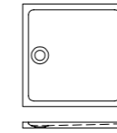
Shower Tray - Single (SB452) 900 W x 900 D x 50 H
