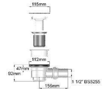
Neo Angle Tray Waste Dimensions
