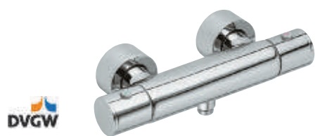
DVGW 54926 Thermostat battery for shower exposed, handle with 50% quantity limiter, safety cut-off at 38 °C, intrinsically safe against backflow
