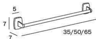
A2218C CR cm 65 x 7H x 7 ●—● cm 60 ● mm 16
