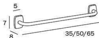
A2290C CR cm 65 x 7H x 8 ●—● cm 60 ● mm 16
