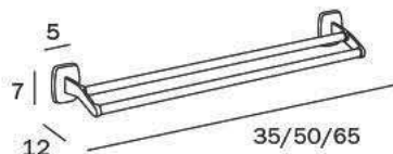
A2219C CR cm 65 x 7H x 12 ●—● cm 60 ● mm 16
