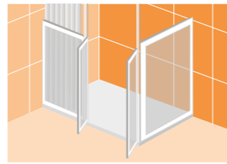
Option D Two fixed half height panels, one 400mm on front, with floor to ceiling poles with one door hung from each panel
