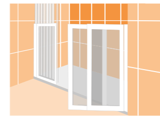
Option 3 One fixed half height 400mm panel with floor to ceiling pole and one sliding door hung from opposite wall
