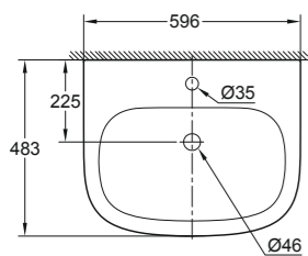
39 337 000 39 337 00H* Countertop basin 60 cm
