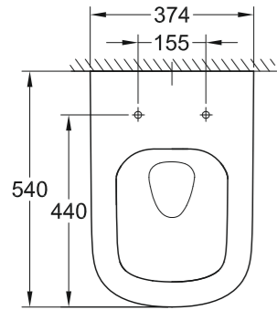
39 328 000 39 328 00H* Wall hung WC, wash down
