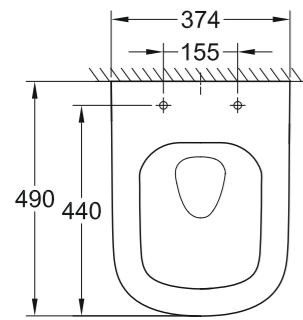
39 206 000 39 206 00H* Compact wall hung WC, wash down
