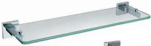
Square Glass Shelf SQ SHELF C Chrome £51.50 Height 48mm Width 467mm Depth 135mm
