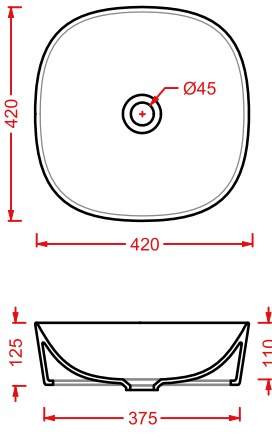
GHL001 GHOST 42 lavabo appoggio countertop washbasin
