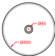
COL001 COGNAC 42 lavabo appoggio countertop washbasin
