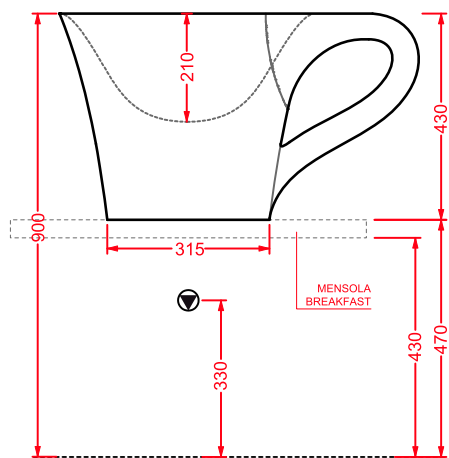
OSL005 CUP lavabo appoggio countertop washbasin
