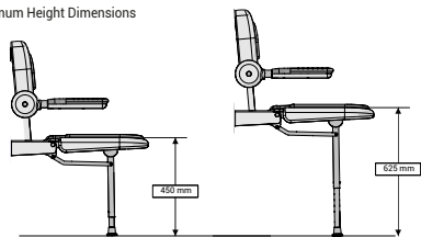
Maximum Height Dimensions
