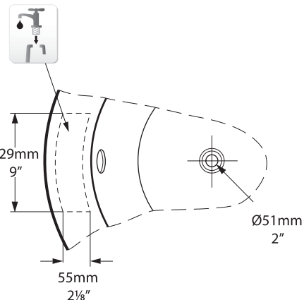
Rim detail
