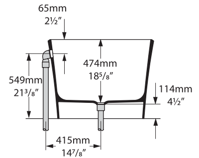
Section BB Shown with K17 waste kit
