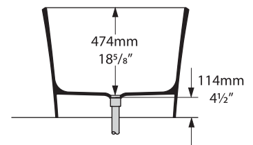
Section BB Shown with K12/K40 waste kit
