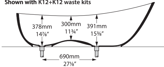
Section AA Shown with K12+K12 waste kits
