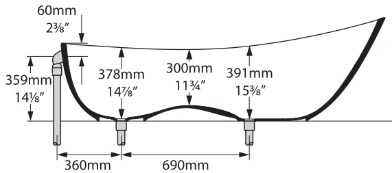
Section AA Shown with K12+K12 waste kits
