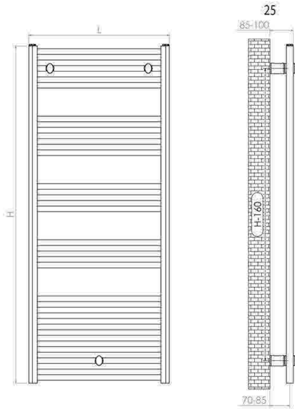
FRONT VIEW
